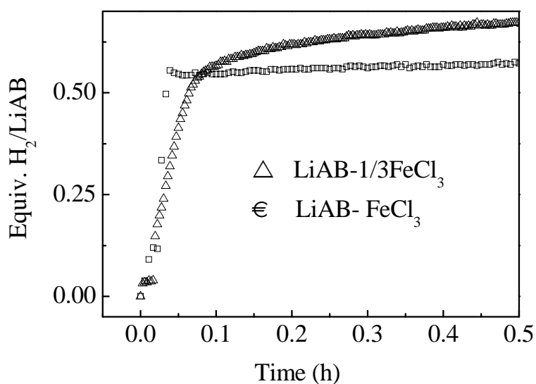
Figure S1. Time-dependent hydrogen desorptions from LiAB-1/3FeCl 3 and LiAB-FeCl 3 THF solutions at ambient temperature within a narrowed time scale (0-0.5 h).
