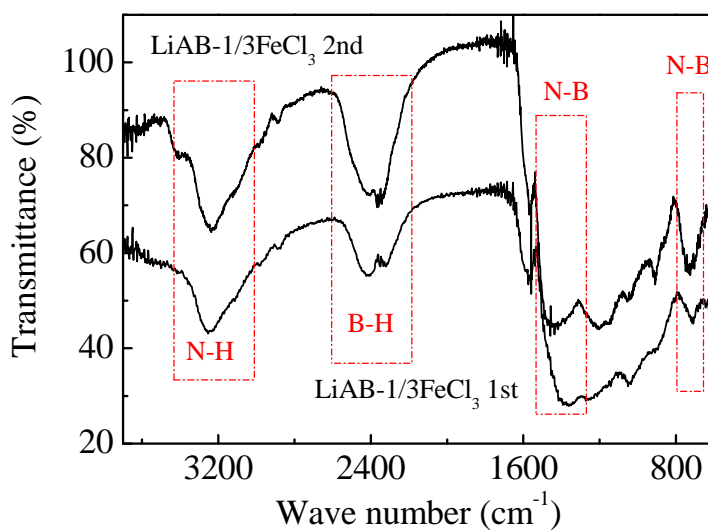
Figure S2. FTIR spectra of precipitates of LiAB-1/3FeCl 3 collected at the end of first and second desorption steps
