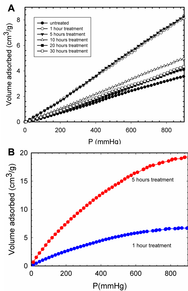
Figure 1 Evidence of CO 2 and H 2 adsorption on the different samples; A: CO 2 adsorption (volume - STP) measured at 293K on the series of samples; and B: H 2 volume adsorbed at 77 K for the 1 h and 5 h plated samples
