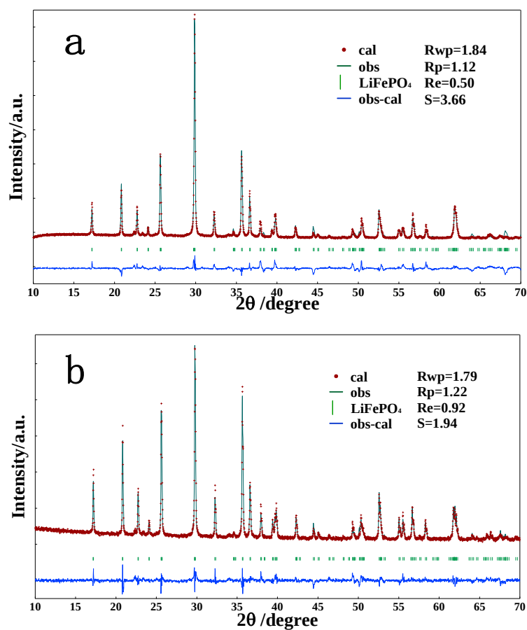
XRD patterns of \text{LiFePO}_4 synthesized at (a) 120°C and (b) 160°C by Rietveld refinement.
