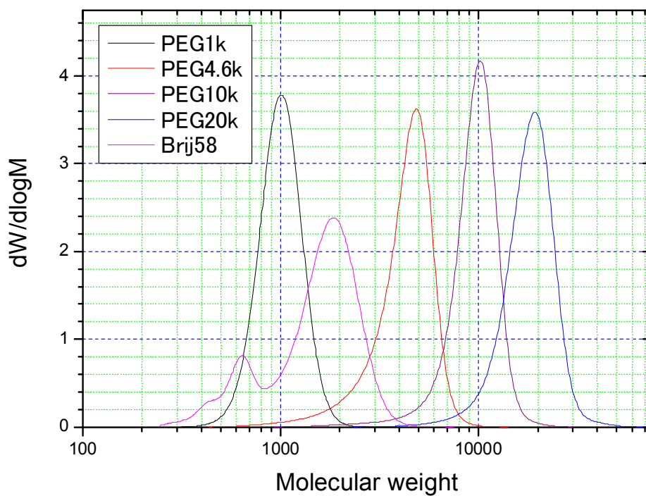
Fig. S1 Molecular weight of spectra of PEG and Brij solutions.
