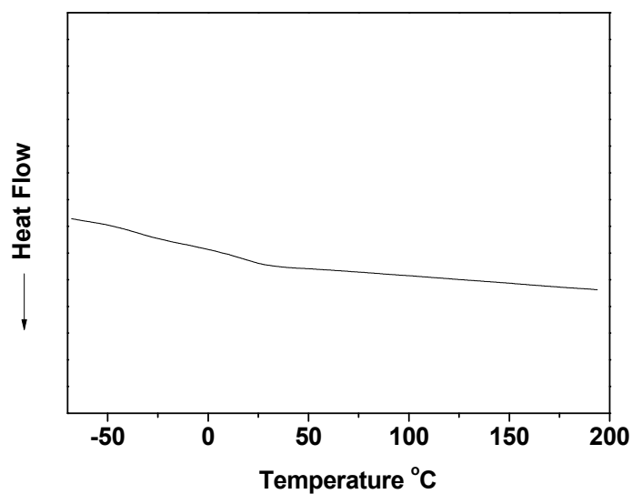
Figure S2. DSC curve of block copolymer during the second heating at a rate of 10 °C/min. The second heating was after the samples were heated to 200 °C and then cooled to -80 °C at the rate of 20 °C/min.
