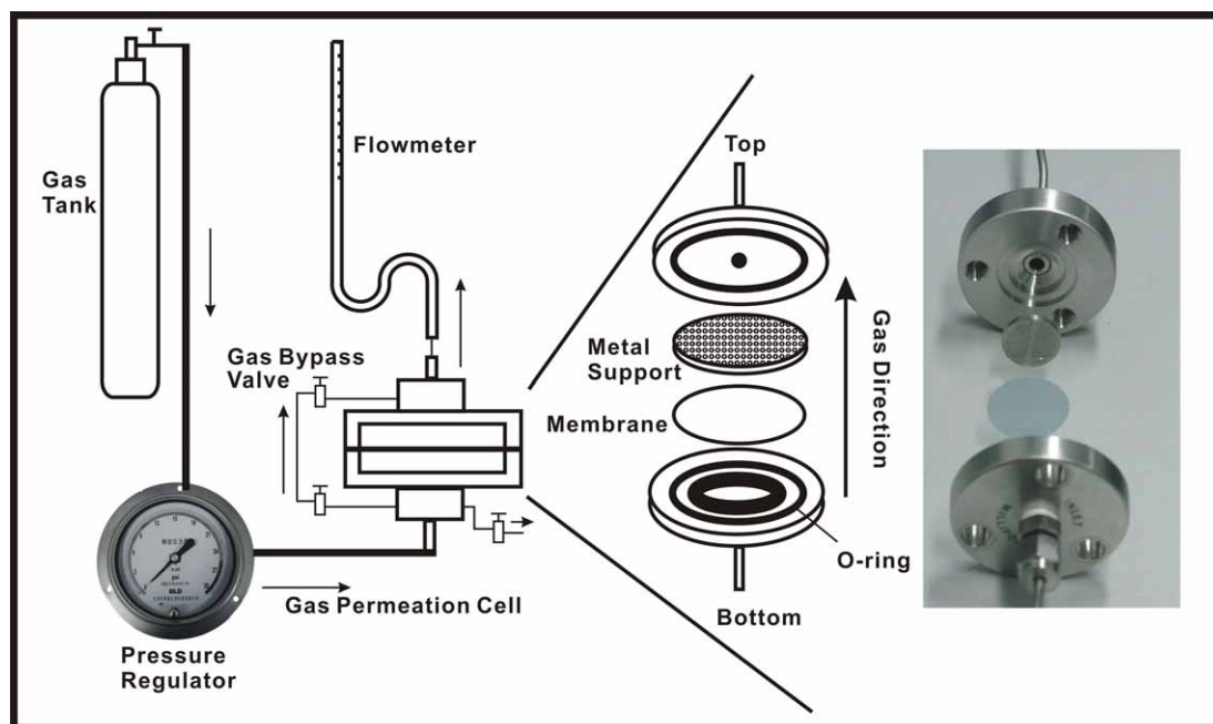
Figure S3. Schematic representation of the home-built permeation apparatus (not drawn to scale).
