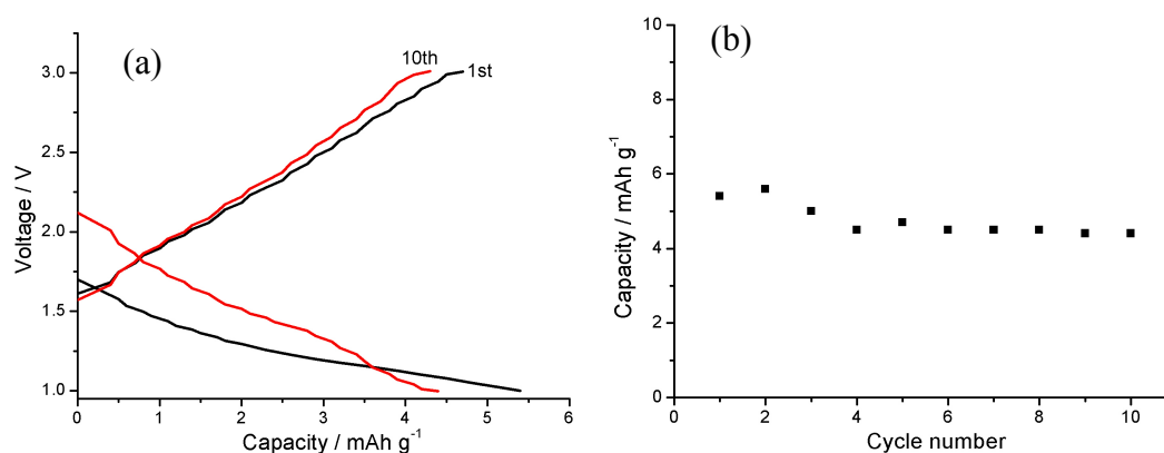
Fig. S1 (a) 1 st and 10 th charge/discharge curves and (b) cyclic performance of CNFs at 1C.
