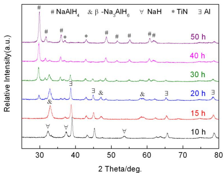
Fig. S1 XRD patterns of the as-synthesized TiN-doped \text{NaAlH}_4 at different milling times.
