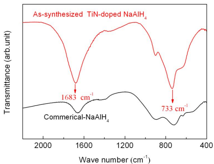
Fig. S2 FTIR spectra of as-synthesized TiN-doped \text{NaAlH}_4 and commercial- \text{NaAlH}_4 .
