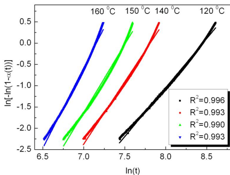
Fig. S3 JMA plots for the first-step isothermal dehydrogenation.
