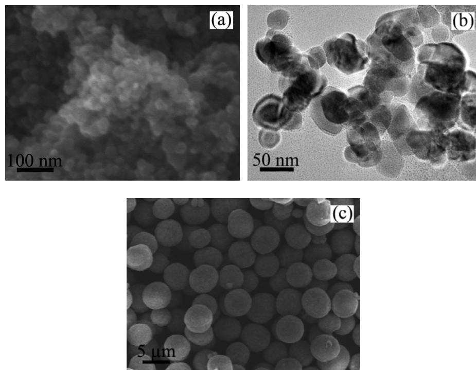
Fig. S1 (a) SEM and (b) TEM image of nanosized \alpha -Fe 2 O 3 , (c) SEM image of micron-sized \alpha -Fe 2 O 3 .
