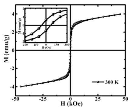
Fig. S3 Hysteresis loop of MNFSSs measured at 300 K. Inset: The enlarged magnetization curve between -300 and 300 Oe.
