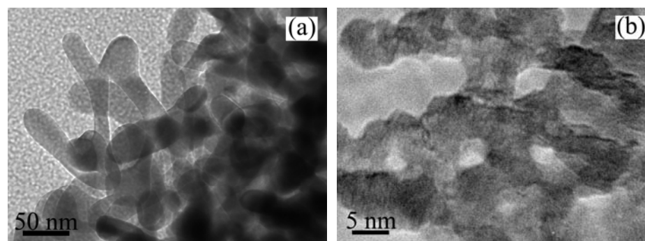
Fig. S2 (a) TEM image of MNFSSs' surface, (b) pore distribution (size about 2 nm) in MNFSSs.
