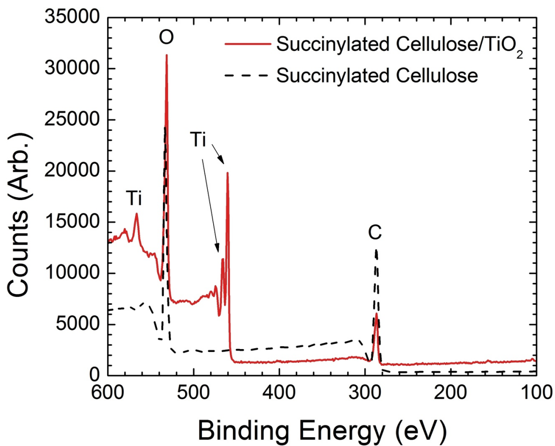
Figure S2. Example XPS spectra of succinylated cellulose (dashed black line) and P-25 loaded succinylated cellulose (red line).
