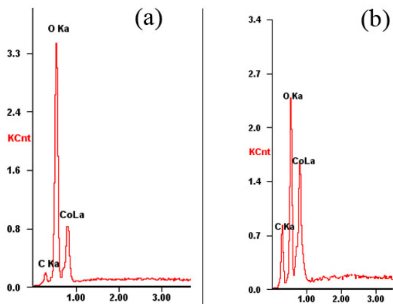
Fig. S1 EDS of \text{Co}_3\text{O}_4 nanowire arrays (a) before and (b) after carbon coating.
