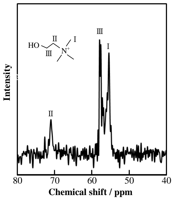
Figure 1S. ^{13}\text{C} CP MAS NMR spectrum of HUS-4 (Sample 7).
