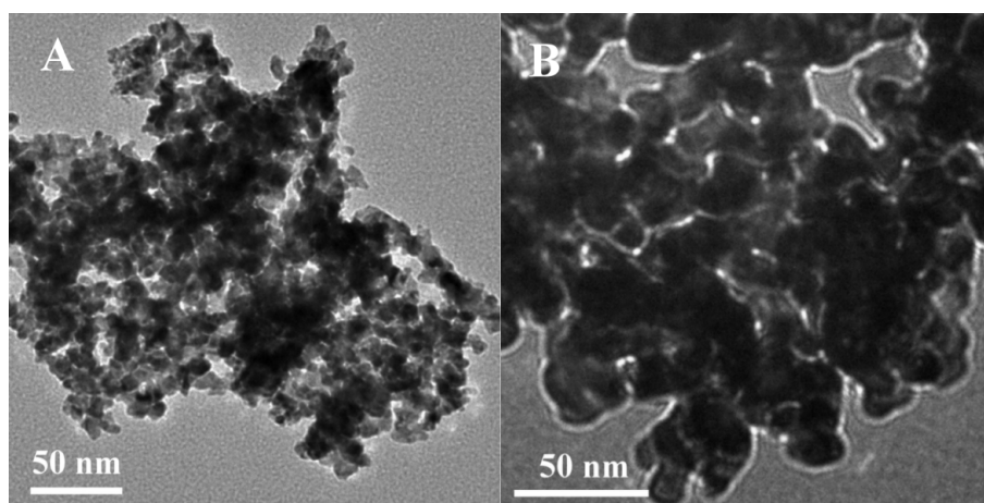
Fig. S4. TEM images of E-TEK Pt black (A) before and (B) after the accelerated durability test.
