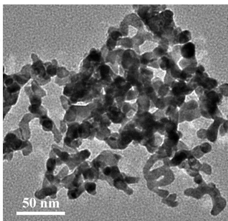
Fig. S3. TEM image of Pt-3NCNWs after the accelerated durability test.
