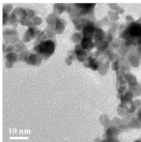
Fig. S1. TEM image of the obtained Pt nanostructures in the absence of NaI.
