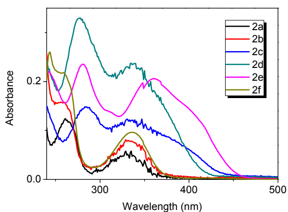
Fig. S1 UV-Vis absorption spectra Schiff base ligands in CH 2 Cl 2 (1.0 × 10 -5 M).
