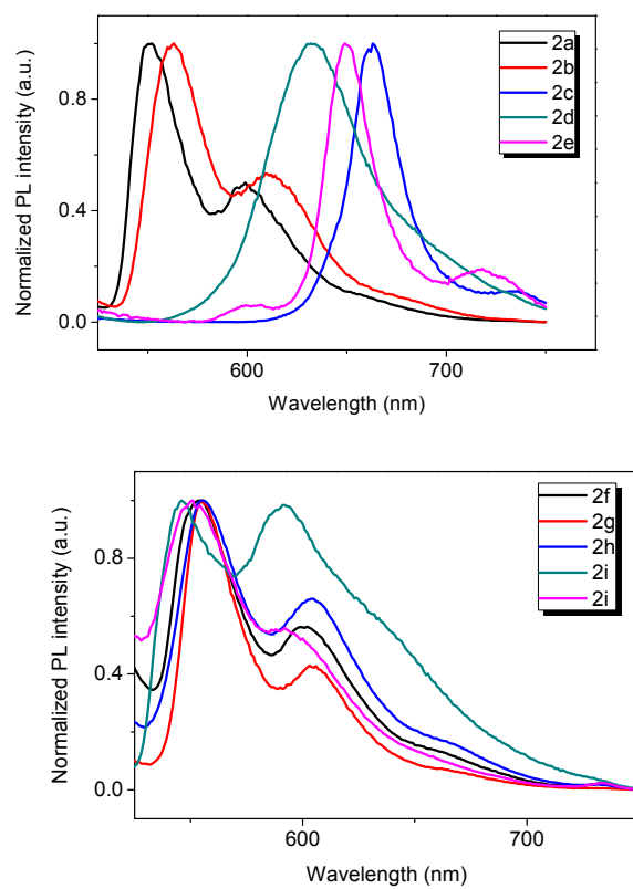
Fig. S2 Emission spectra of Pt(II) Schiff-base complexes 2a — 2j in CH 3 CN ( 1.0 \times 10^{-5} M) at 77 K.
