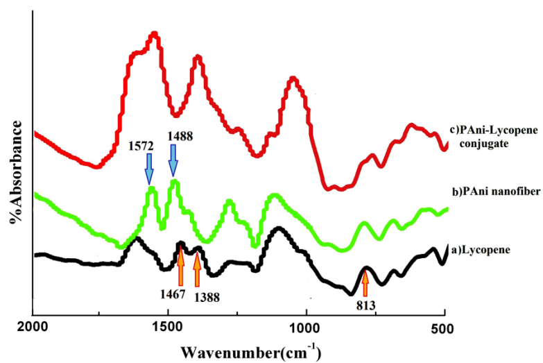
Fig. S1 FTIR spectra of a) lycopene, b) PANi nanofiber and c) PANi-lycopene conjugated system
