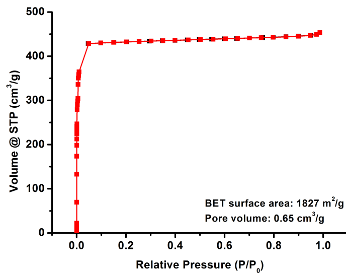
Figure S4. N 2 adsorption-desorption isotherm of the ZIF-8 microcrystals
