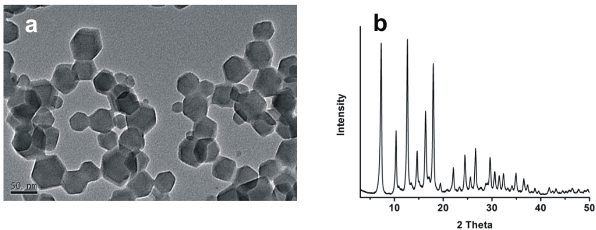
Figure S2. TEM image (a) and XRD pattern (b) of the ZIF-8 nanocrystals
