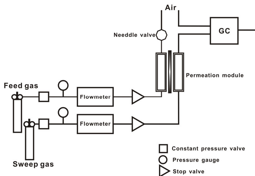
Figure S1. Illustration of the measurement equipment for gas separation
