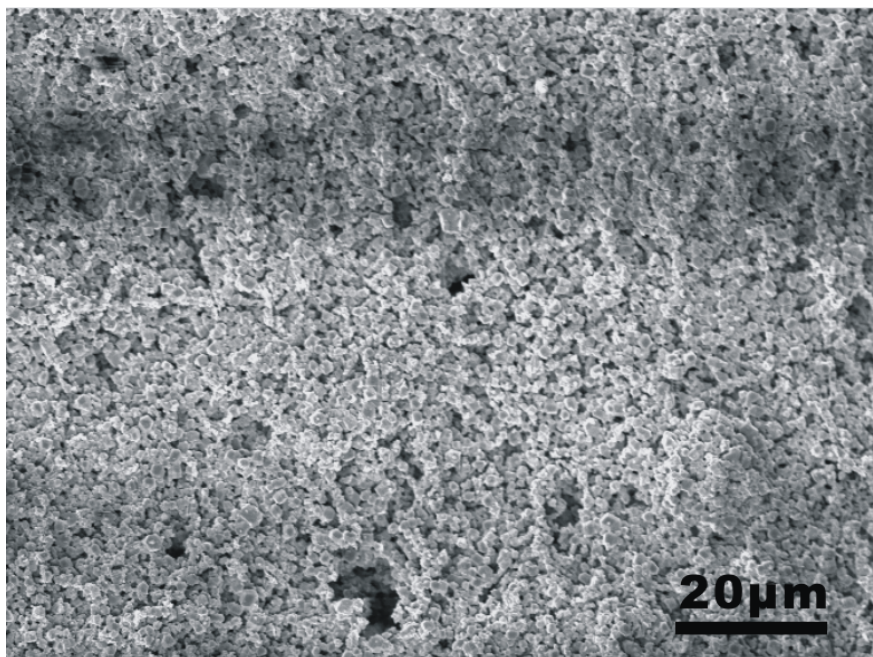
Figure S5. SEM image of the synthesized ZIF-8 membranes after removal of the polymer fibers by THF
