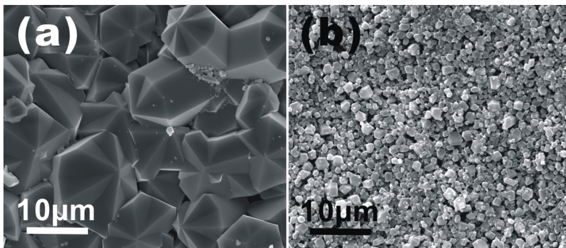
Figure S3. SEM images of the ZIF-8 membrane prepared by using sodium formate in growth solution (a) and without the addition of sodium formate in growth solution (b).
