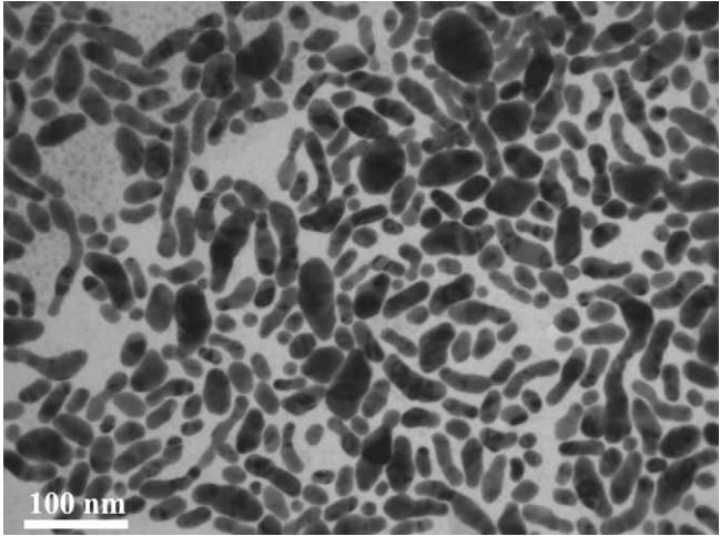
Fig. S3 TEM images of the obtained AuPt NPs without the addition of \text{H}_2\text{PdCl}_4 .
