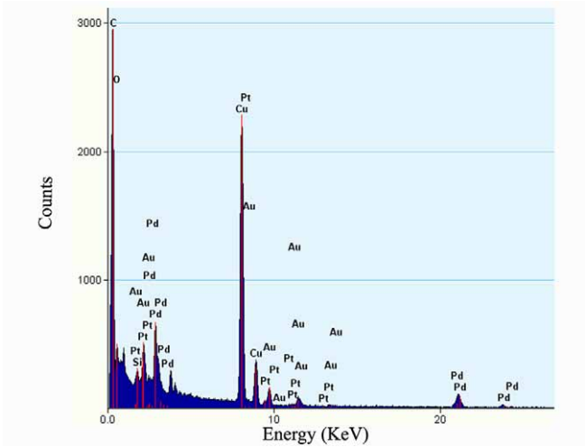
Fig. S2 EDX spectroscopy of the obtained AuPtPd ANWs.
