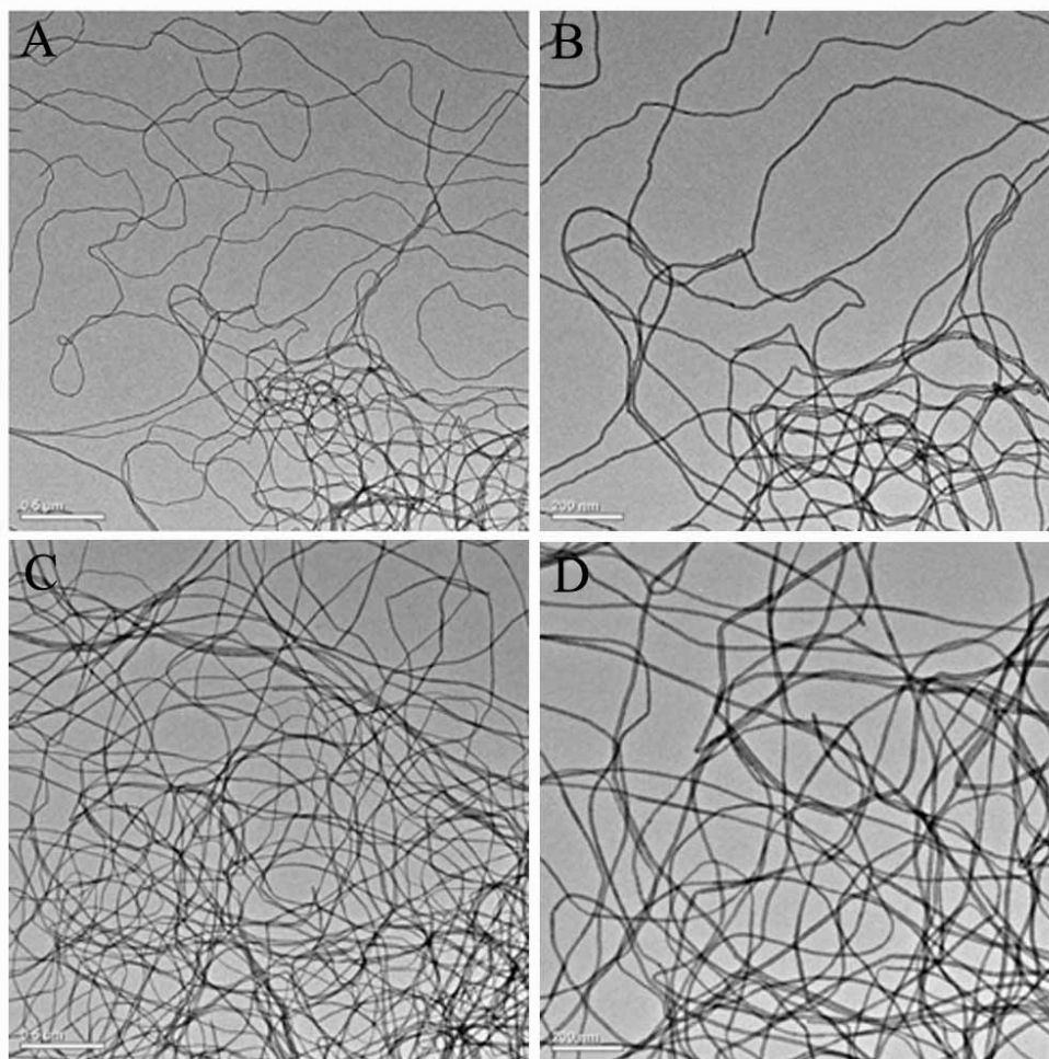
Fig. S1 TEM images of the bimetallic PtPd (A, B) and AuPd (C, D) ANWs.
