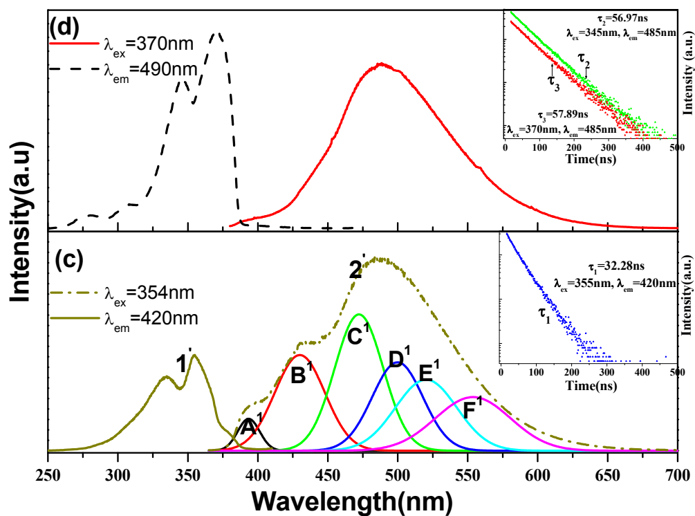
Fig. PL and PLE spectra of phosphors \text{Ba}_2\text{Y}(\text{BO}_3)_2\text{Cl}:3.0\%\text{Ce}^{3+} at LTH. Insets: The decay curves of \text{Ce}^{3+} at different sites displayed on a logarithmic intensity scale at LTH.
