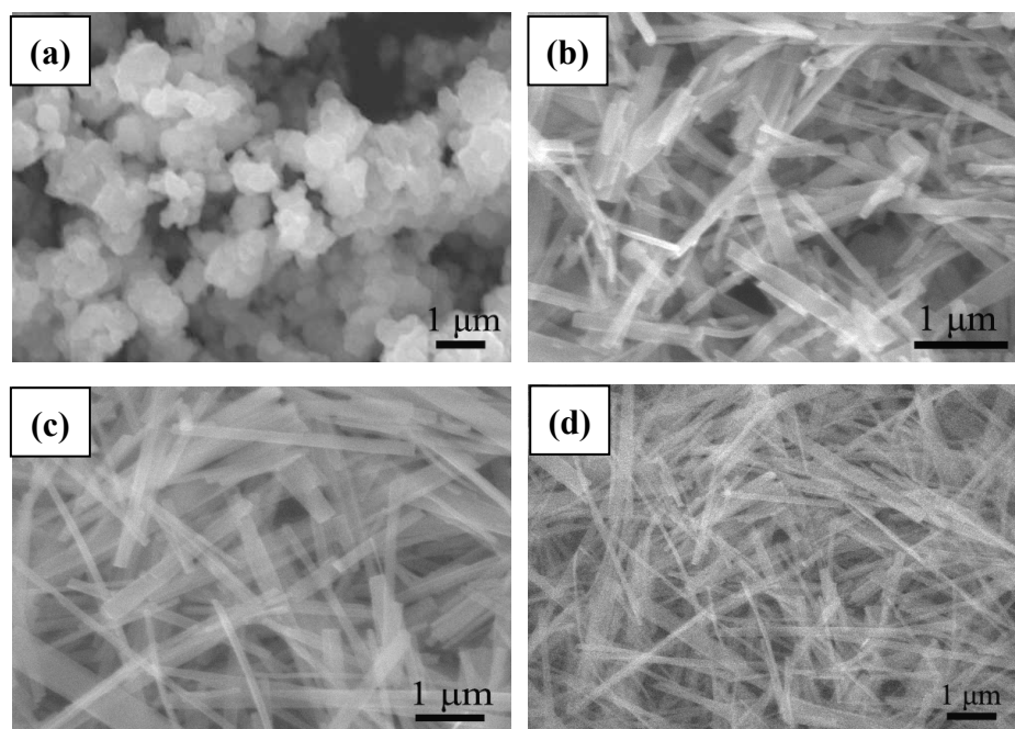
Figure S1. SEM images of (a) raw anatase TiO 2 particles and the synthesized (b) hydrogen titanate nanosheets, (c) uniform anatase TiO 2 nanosheets, (d) architected anatase TiO 2 nanosheets.
