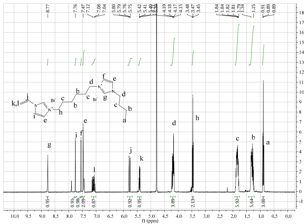
Figure S3. 1 H NMR (D 2 O) spectrum of [BVIm][HIm][Br].
