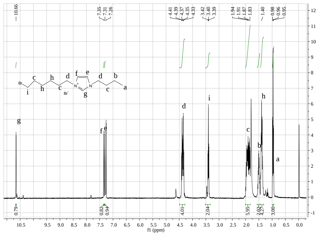
Figure S2. 1 H NMR (CDCl 3 ) spectrum of [BrHBIIm][Br].
