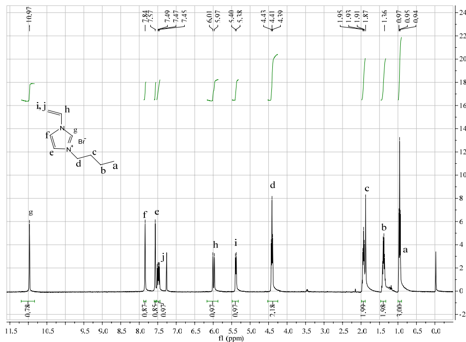
Figure S1. 1 H NMR (CDCl 3 ) spectrum of [BVIm][Br].
