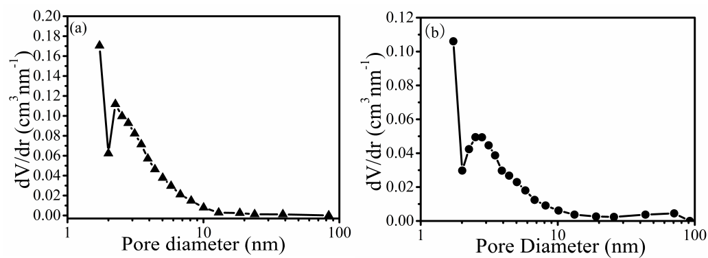
Figure 2 The BJH pore size distribution curves of the IPC-I(a) and IPC-II(b).
