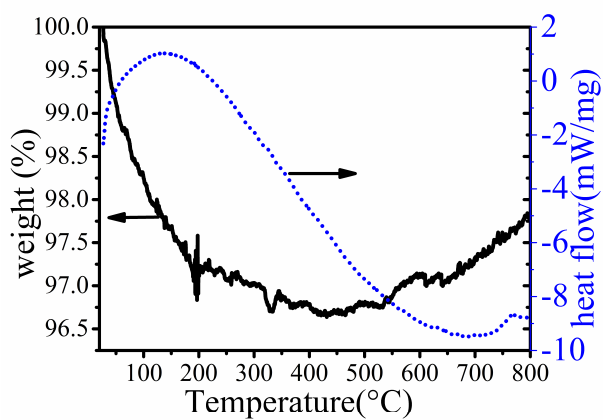
Figure 3 The TG/DTA curves of IPC-I.
