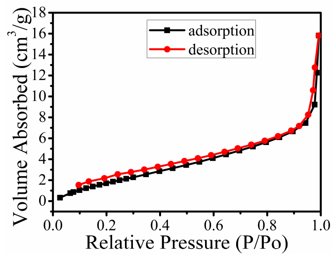
Figure 1 The nitrogen adsorption-desorption isotherms of the IPC-II.
