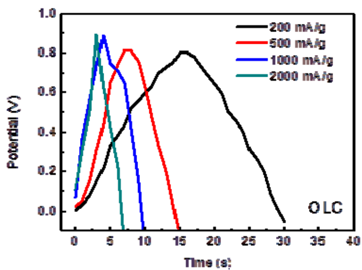
Fig. S1 Charge/discharge curves of pure onion-like carbon electrode at different current densities.
