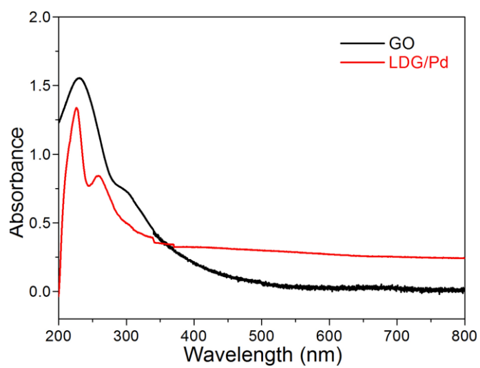
Fig. S2 UV-vis absorption spectra of GO and LDG/Pd.
