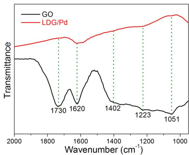
Fig. S1 FT-IR spectra of GO and LDG/Pd.
