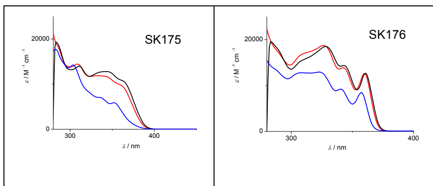
Figure S1. Absorption spectra of the compounds in TL(black) , DCM(red) and MeOH(blue).
