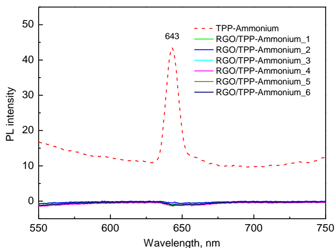
Figure S1. PL spectra of the multiple-bilayered RGO/TPP-ammonium films.
