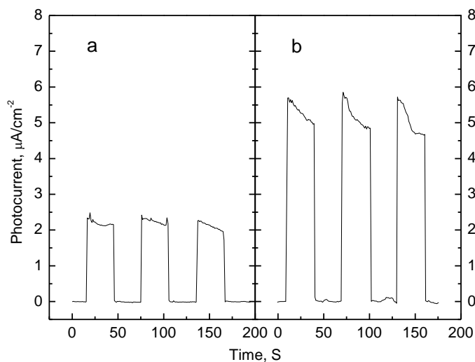
Figure S2. Typical photocurrent curves of (a) a one-bilayered RGO/TPP-ammonium film and (b) a six-bilayered RGO/TPP-ammonium film.
