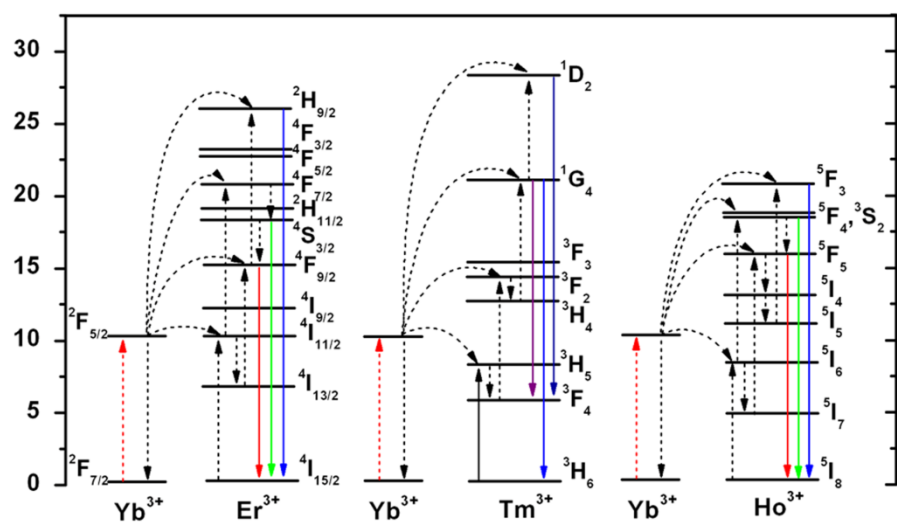
Figure S3. Schematic energy level diagrams showing typical UC processes for Yb 3+ , Er 3+ , Tm 3+ and Ho 3+ .
