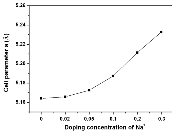
Figure S1. The cell parameter as a function of the \text{Na}^+ doping concentrations ( x ).
