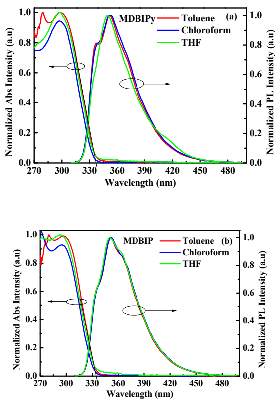
Figure S1. The PL spectrum of MDBIP and MDBIPy in different solvent.
