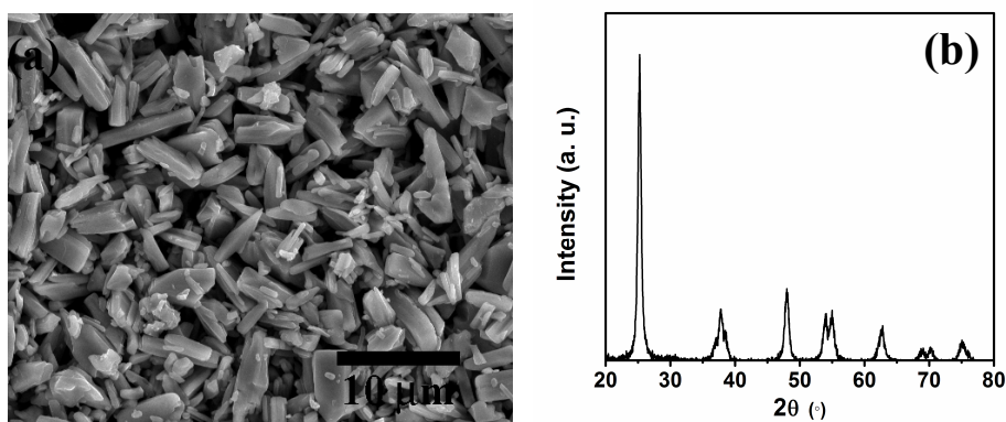
Fig. S1 FE-SEM image (a) and XRD pattern (b) of \text{TiO}_2 microrods prepared by calcining titanium glycolate precursor at 450 ^\circ\text{C} .
