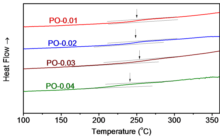
Figure S2. DSC curves of the polymers.
