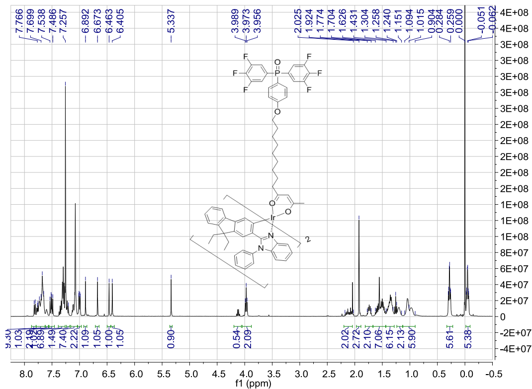
Figure S8. ^1\text{H} NMR spectrum of Y-MON.
