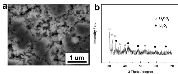
Fig. S3 SEM image (a) and XRD pattern (b) of the discharge product after 2 nd discharge.
