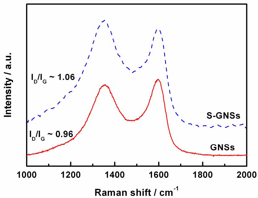
Fig. S2 Raman spectroscopy of S-GNSs and GNSs.
