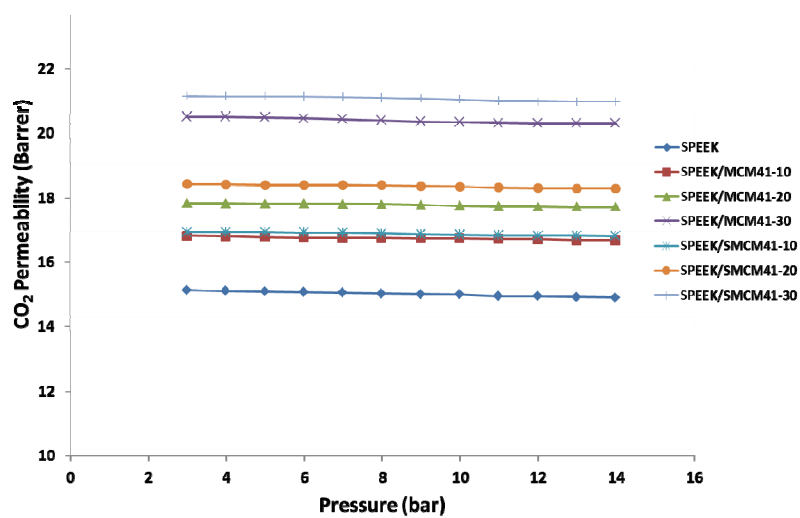
Fig. S1 Pure gas (CO 2 ) permeability for MMMs as a function of upstream pressure.
