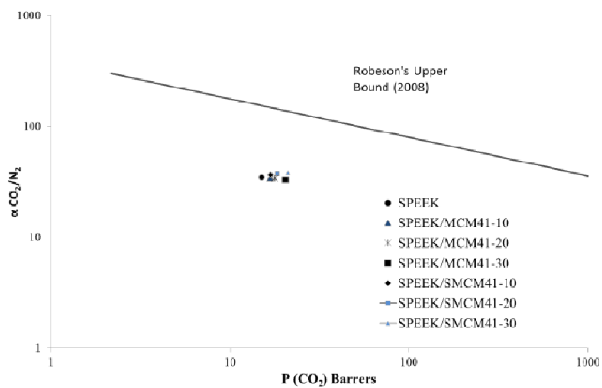
Fig. S2 Robeson plot of CO 2 /N 2 performance.
