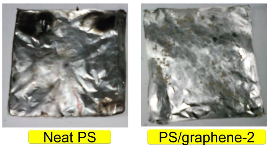
Fig. 10 PS and PS/graphene-2 composite (containing 2 wt% graphene) after cone test; no char is formed with the PS/graphene-2 composite. The samples are referred to prior work (Reference 9: C. L. Bao, L. Song, C. A. Wilkie, B. H. Yuan, Y. Q. Guo, Y. Hu and X. L. Gong, J. Mater. Chem. , 2012, 22, 16399-16406.)
