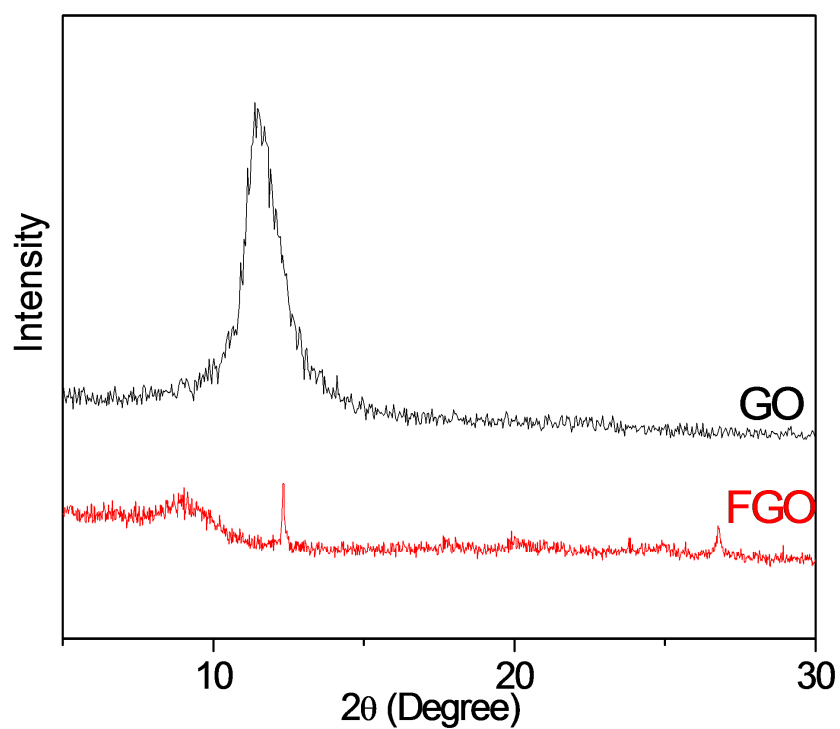
Fig. 3 XRD patterns of GO and FGO
