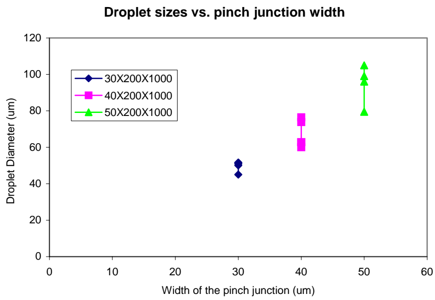
Figure a. Experiment results indicate that droplet sizes are mainly controlled by the width of the pinch junction due to the shear force applied.
