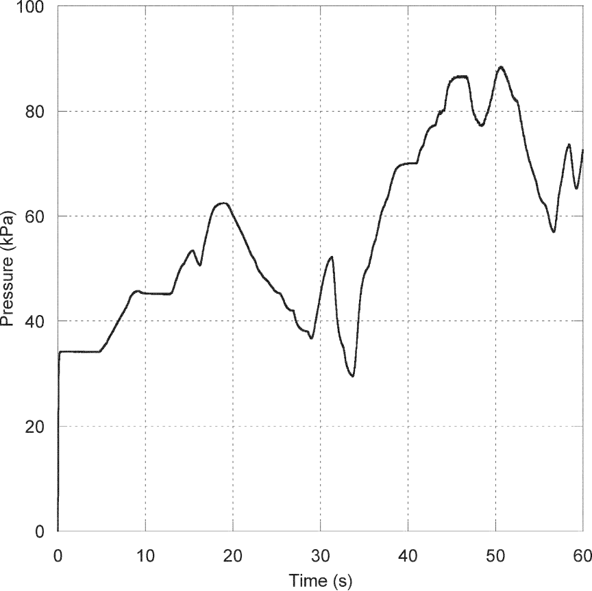
Fig. S1 Arbitrary, time-dependent pressure waveform used to validate flow rate measurement technique.
