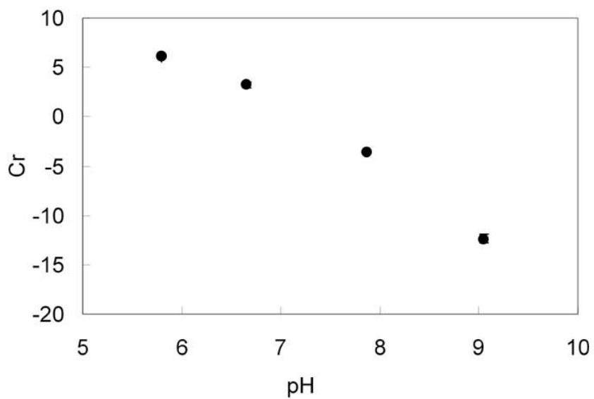
Fig. S1 Calibration result of pH with Cr.
