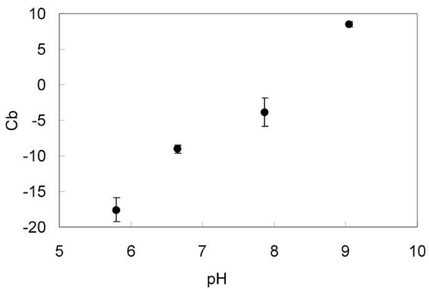
Fig. S2 Calibration results of pH with Cb.
