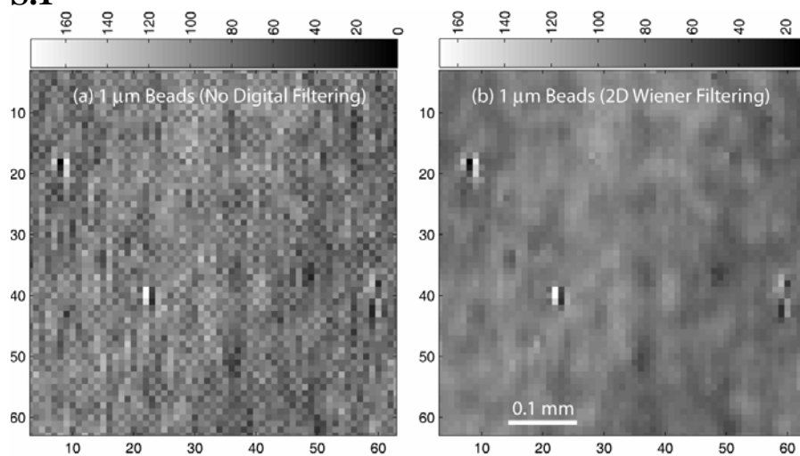
Figure S.1: (a) LUCAS image of 1 μm diameter polystyrene microbeads. (b) 2D Wiener filtering applied to the same image to digitally increase the contrast and SNR of the image.
