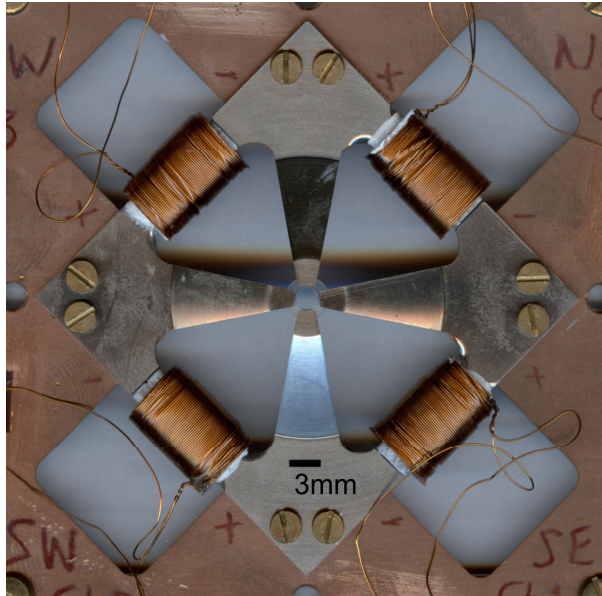
Supplementary Figure: The experimental setup used. It consists of 4 coils and 4 flux guides that concentrate the field in the area of the fluid. The fluid container lies in the centre between the 4 flux guides.
