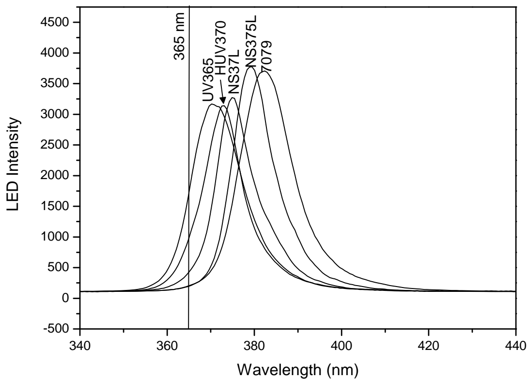
Emission spectra of the LEDs considered for this work
