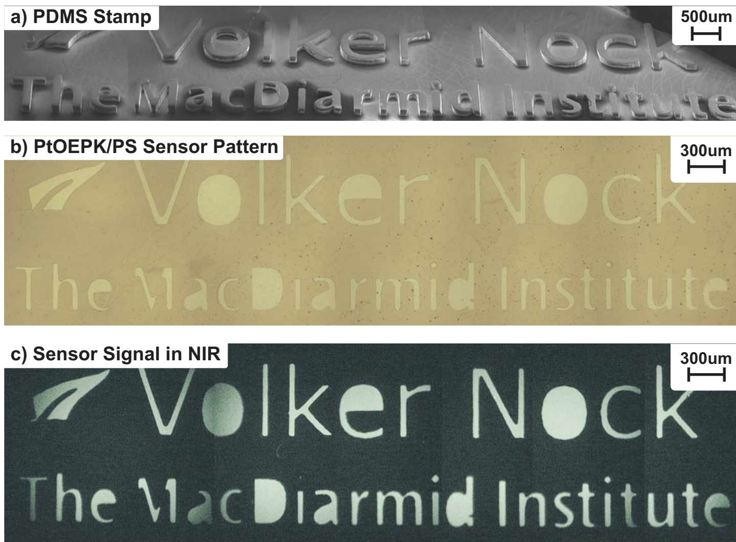
Figure Test pattern replicated in PtOEPK/PS by the fabrication process: (a) SEM micrograph of the PDMS stamp used as mask in the RIE step, (b) DIC image of the pattern in the PtOEPK/PS film after etching, and (c) fluorescent emission in the NIR from the same pattern under illumination with light of 590nm wavelength.
