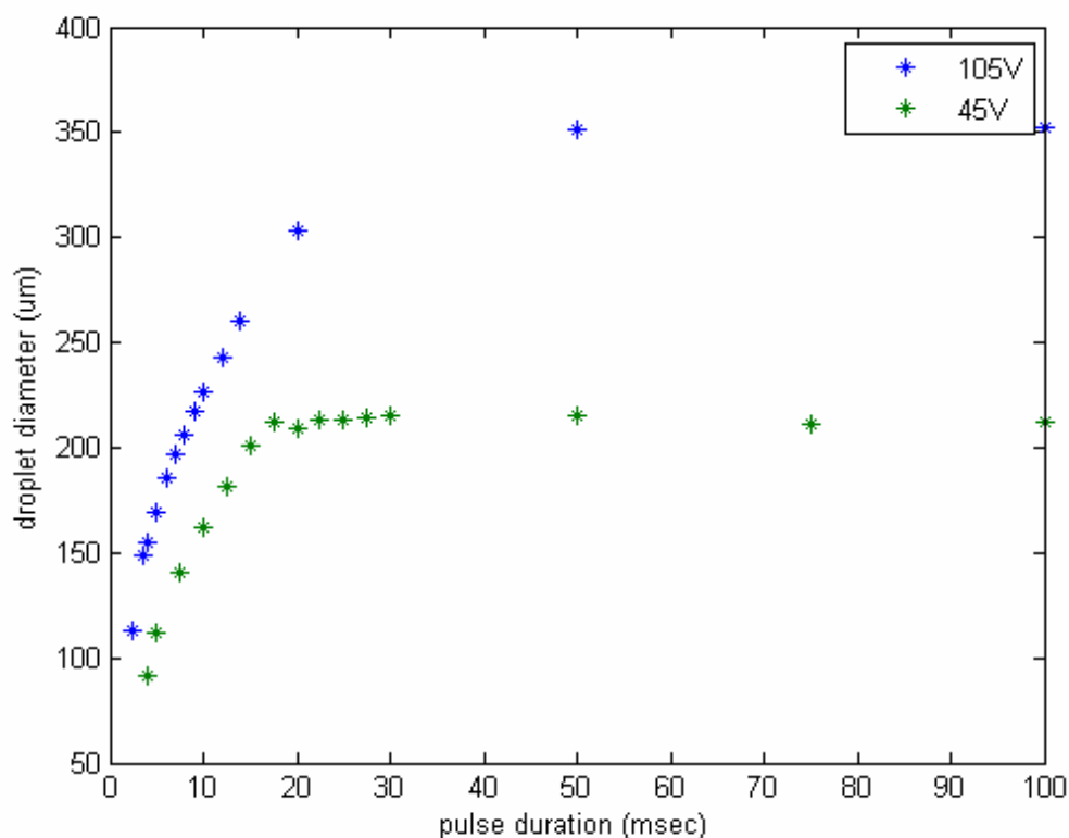
S1: A plot of the mean droplet diameter versus pulse duration as obtained by the cross flow configuration for two amplitudes of 45 and 105 V. The diameter increases rapidly with pulse duration until a critical value is reached whereupon droplet size remains constant.
