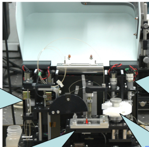
Microchip & TLM
