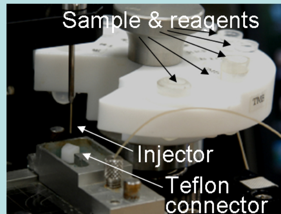
Interface to microchip
