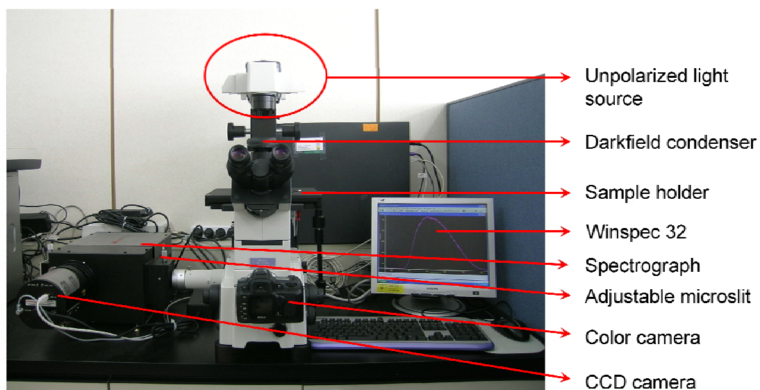
Figure: The colour photograph of the system setup for study of resonant Rayleigh light-scattering response of individual Au nanoparticles.
