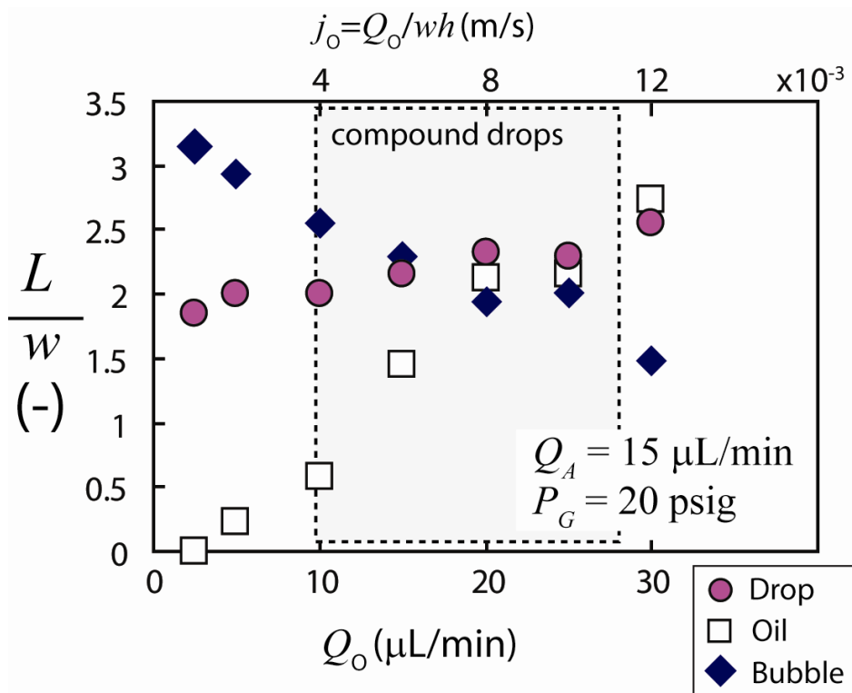
Supplementary Figure S1: Graph of dimensionless bubble length, drop length and oil segment length versus oil volumetric flow rate Q_o , at constant aqueous flow rate Q_A and gas supply pressure P_G .
