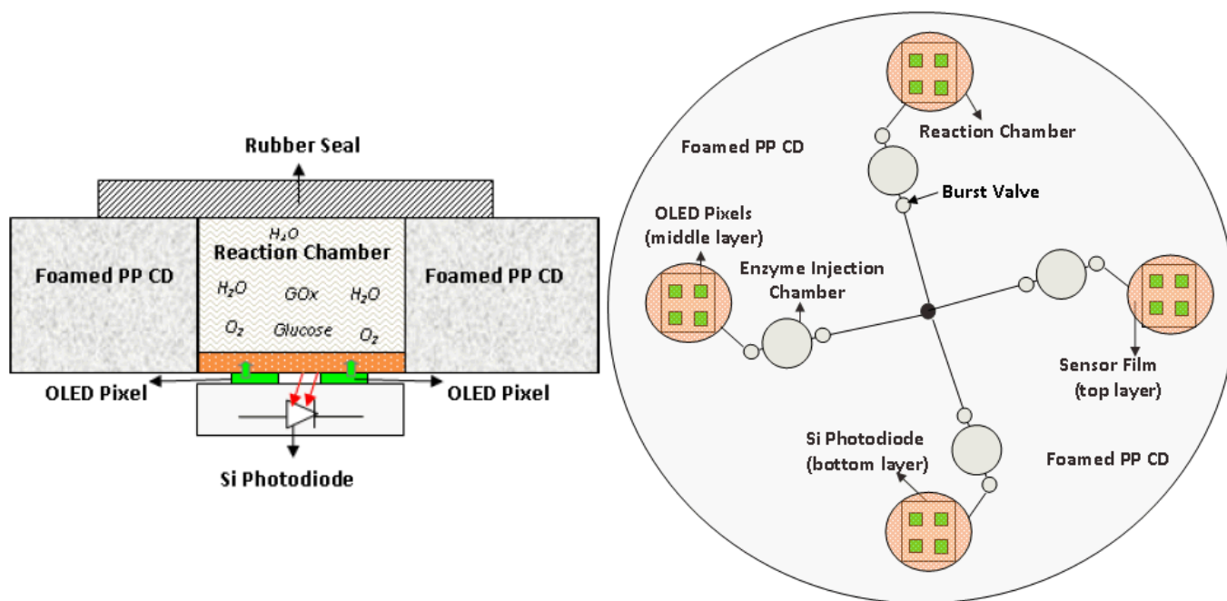
The foamed polypropylene CD-OLED sensing platform. Left: side view of a single sensor; Right: top view of the multiple analyte platform. The drawings are not to scale.
