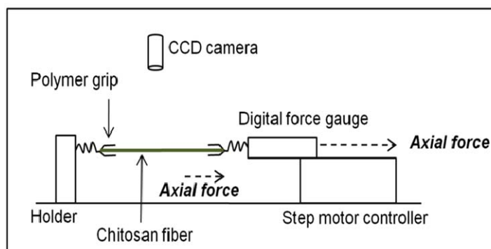
Figure S1. Schematic diagram of axial force measurement system
