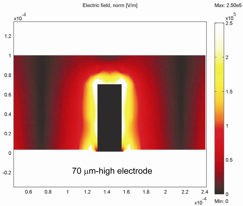
Fig. 2 Electric field on 40 and 70 electrodes
