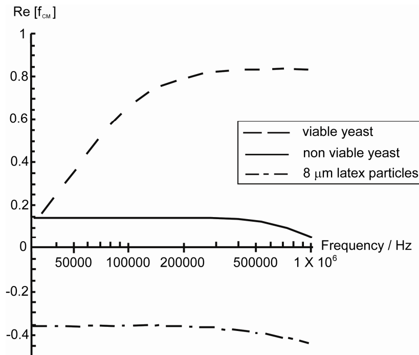
Fig. 1 DEP spectra Latex and Yeast 31.2 uS
