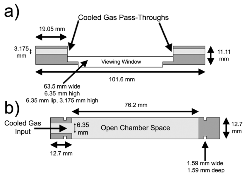
Fig. S1 Detailed measurements of the cooling chamber
