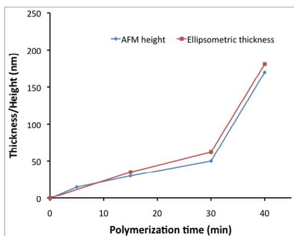
Figure. Comparison of the thickness of the PMAA brush versus the polymerization time measured both by AFM and ellipsometry.
