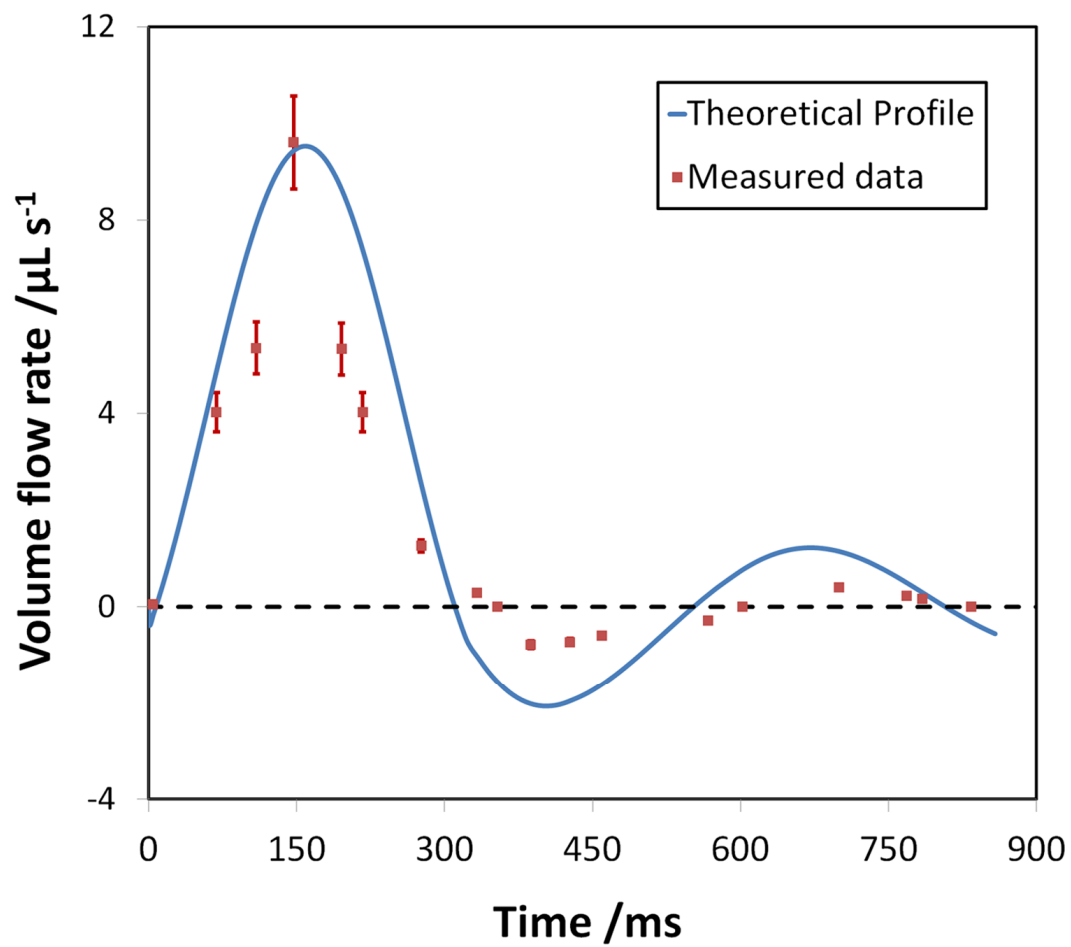
Fig. S1 The measured pulsatile flow profile under the condition of 70 bpm and 15 \text{dyne cm}^{-2} .
