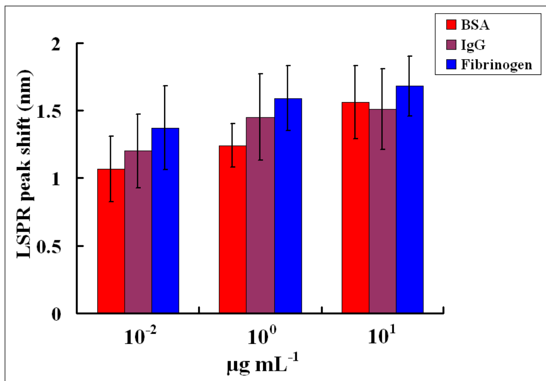
Fig. S1 Non-specific binding of different proteins on the single AuNR surface. The LSPR peak shift of BSA, IgG and IgG increased negligible when the concentrations of BSA, IgG and fibrinogen were increased from 10^{-2} , 10^0 and 10^1 \mu\text{g mL}^{-1} .
