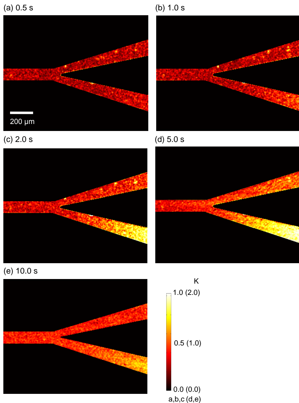
Fig. 6 Images of the temperature difference, \Delta T , at (a) 0.5 s, (b) 1.0 s, (c) 2.0 s, (d) 5.0 s, and (e) 10.0 s after the start of 5 s wire heating, where the image at 0 s is the reference. Note that the color-bar indicates two different scales; 0–1 K is for (a), (b), and (c) and 0–2 K (in parentheses) is for (d) and (e).
